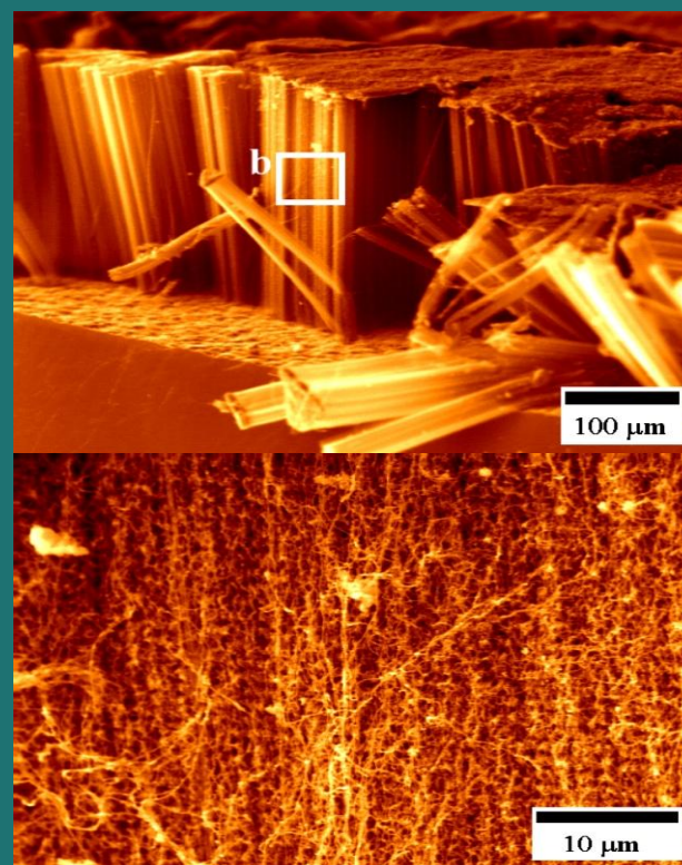
Top and above: Aligned carbon nanotube bundles
